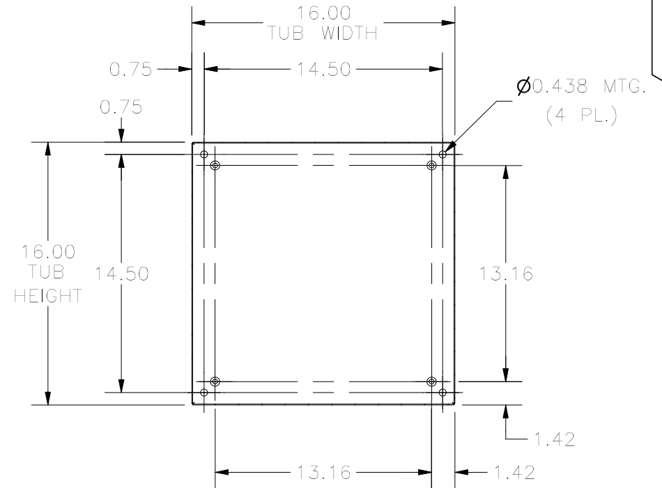
SECTION W-W (INSIDE BACK OF ENCLOSURE)
