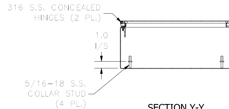
SECTION Y-Y (INSIDE TOP OF ENCLOSURE)
