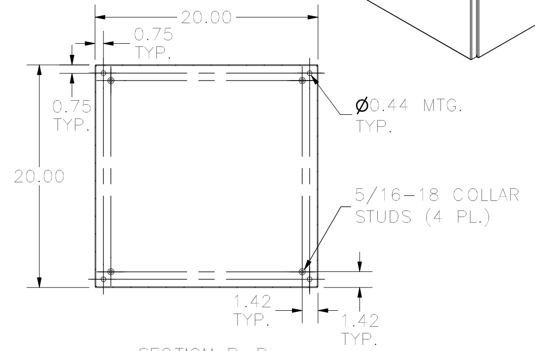
SECTION B-B (INSIDE BACK OF ENCLOSURE)
