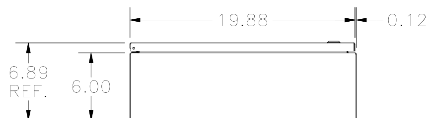
BOTTOM VIEW
