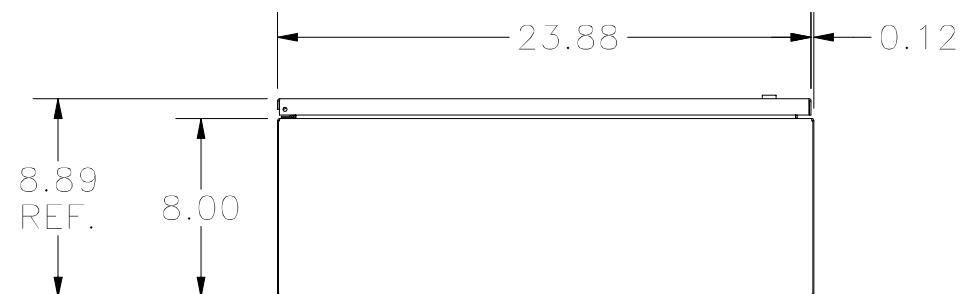
BOTTOM VIEW
