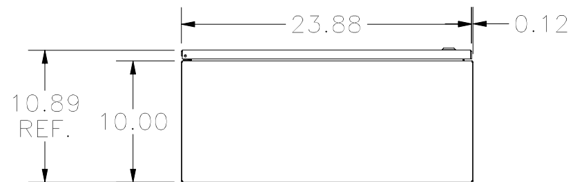
BOTTOM VIEW
