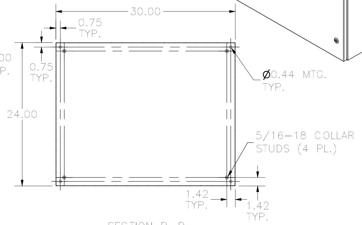
SECTION B-B (INSIDE BACK OF ENCLOSURE)
