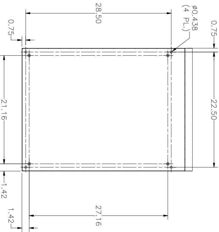
REF. VIEW (DOOR OPEN)
