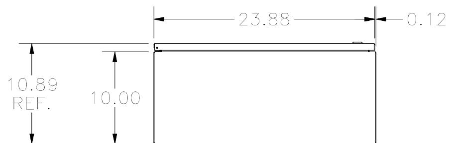
BOTTOM VIEW
