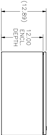
BOTTOM VIEW
