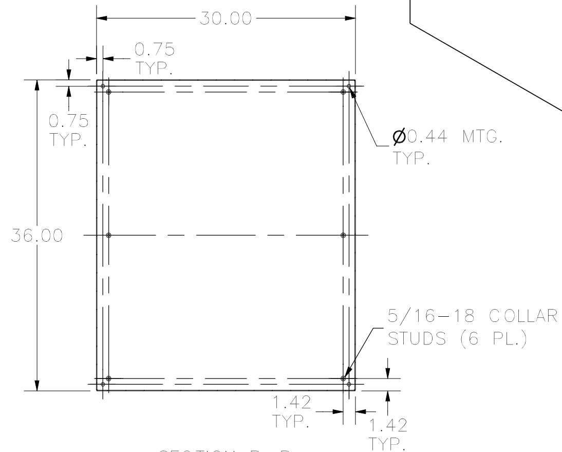
SECTION B-B (INSIDE BACK OF ENCLOSURE)
