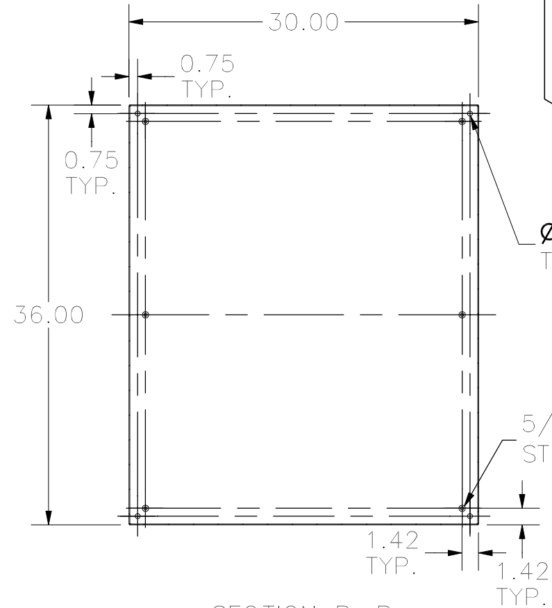
SECTION B-B (INSIDE BACK OF ENCLOSURE)
