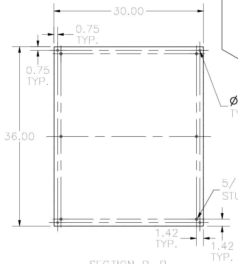
SECTION B-B (INSIDE BACK OF ENCLOSURE)
