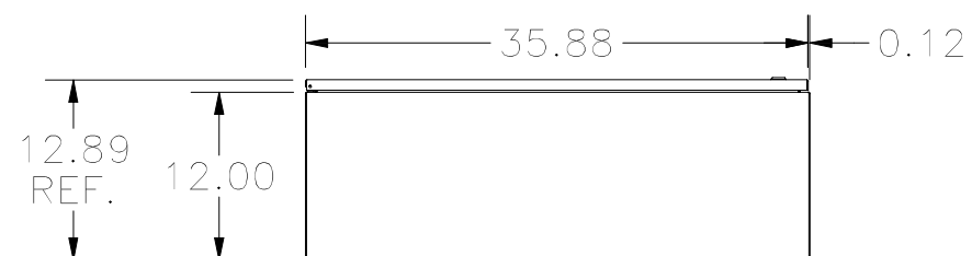
BOTTOM VIEW
