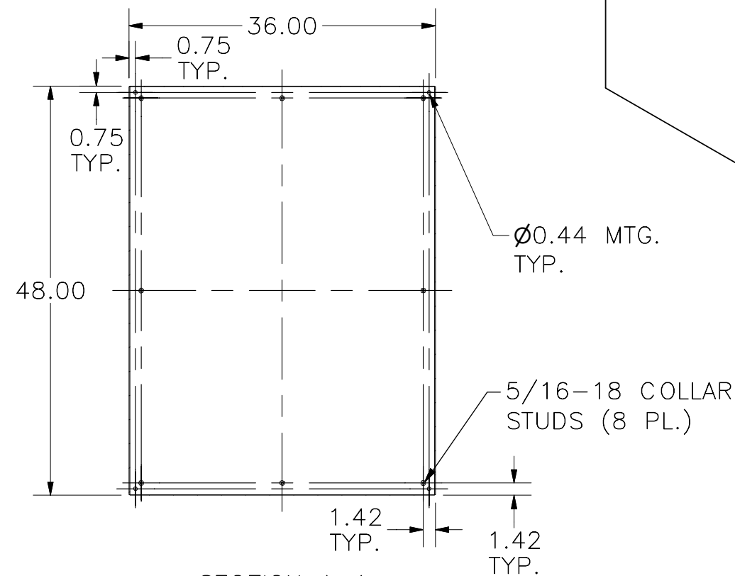
SECTION A-A (INSIDE BACK OF ENCLOSURE)
