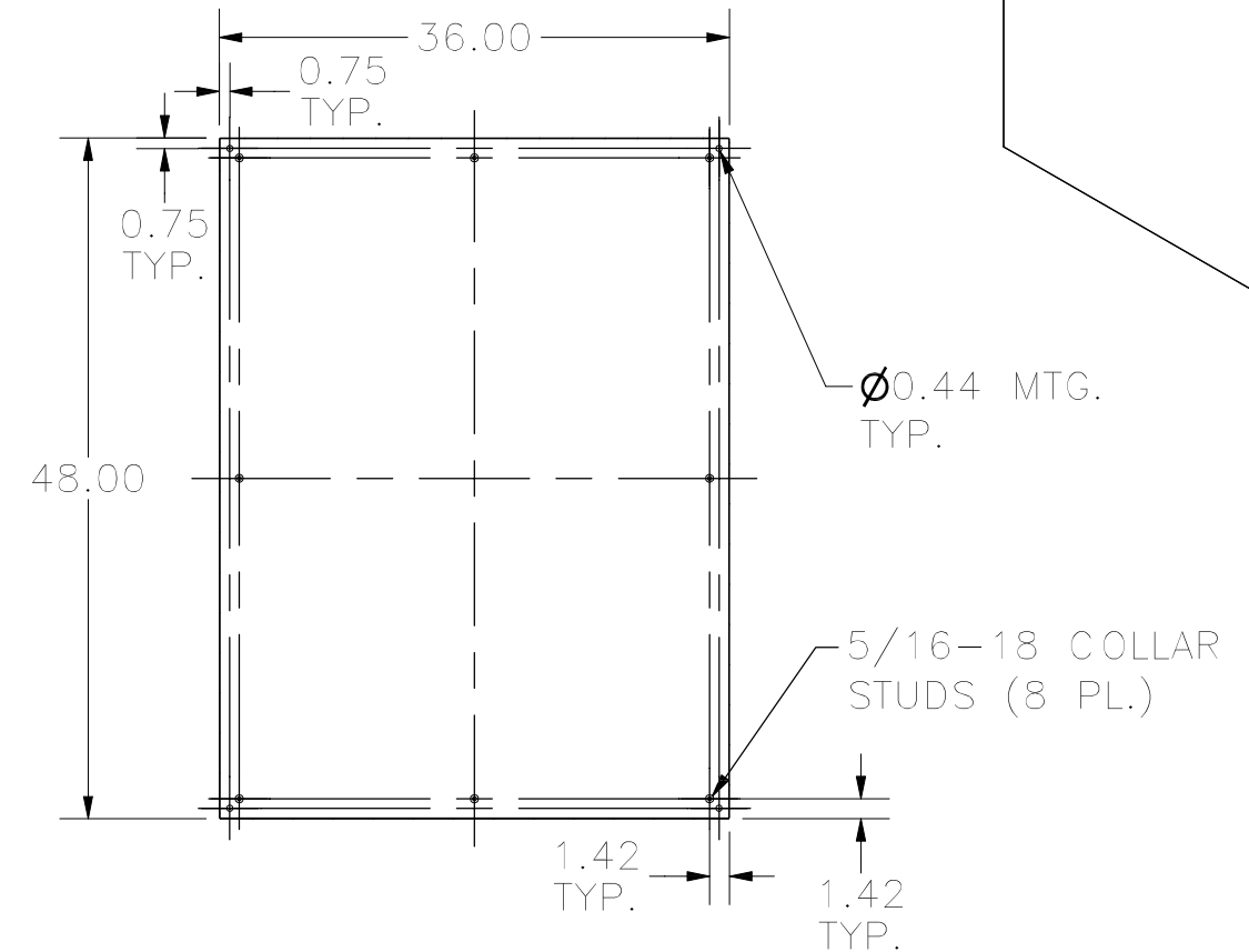
SECTION A-A (INSIDE BACK OF ENCLOSURE)
