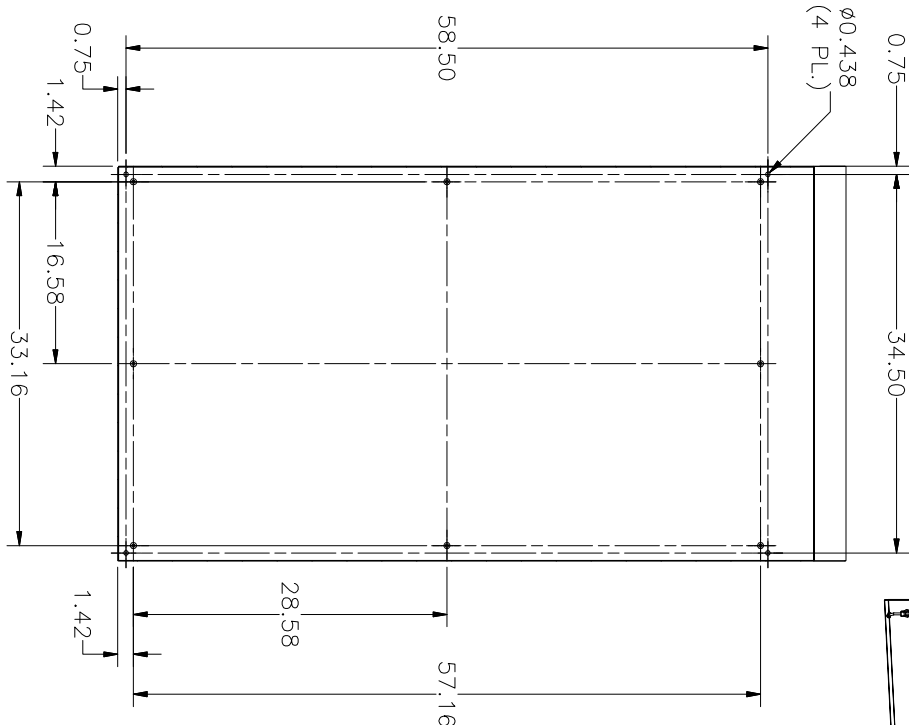
SECTION A-A VIEW (INSIDE BACK OF ENCL.)
