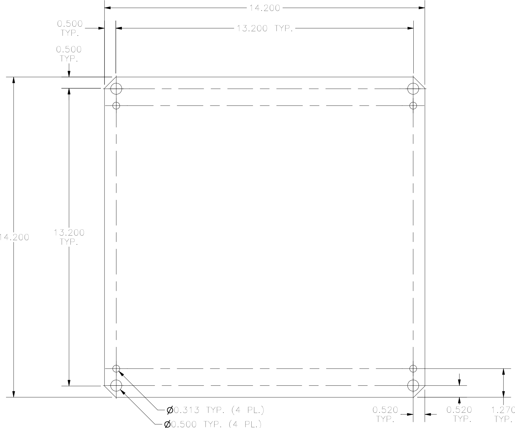
FRONT VIEW
