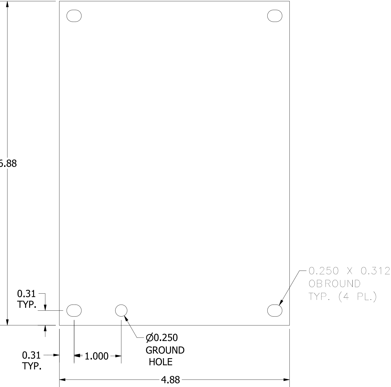
FRONT VIEW
