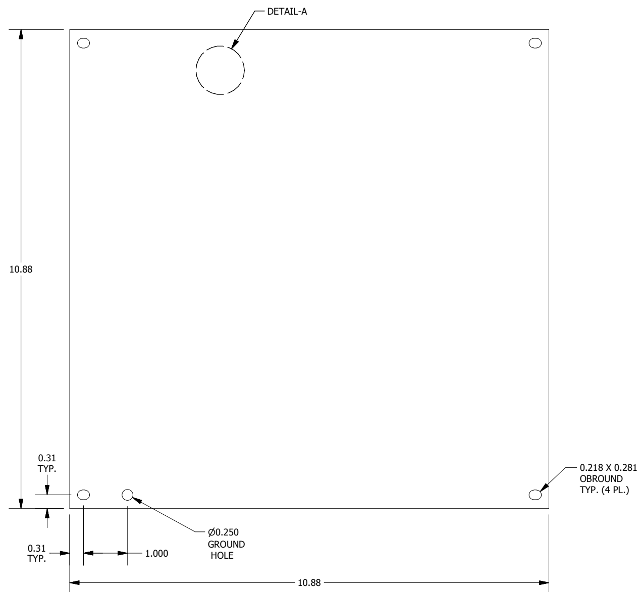
FRONT VIEW
