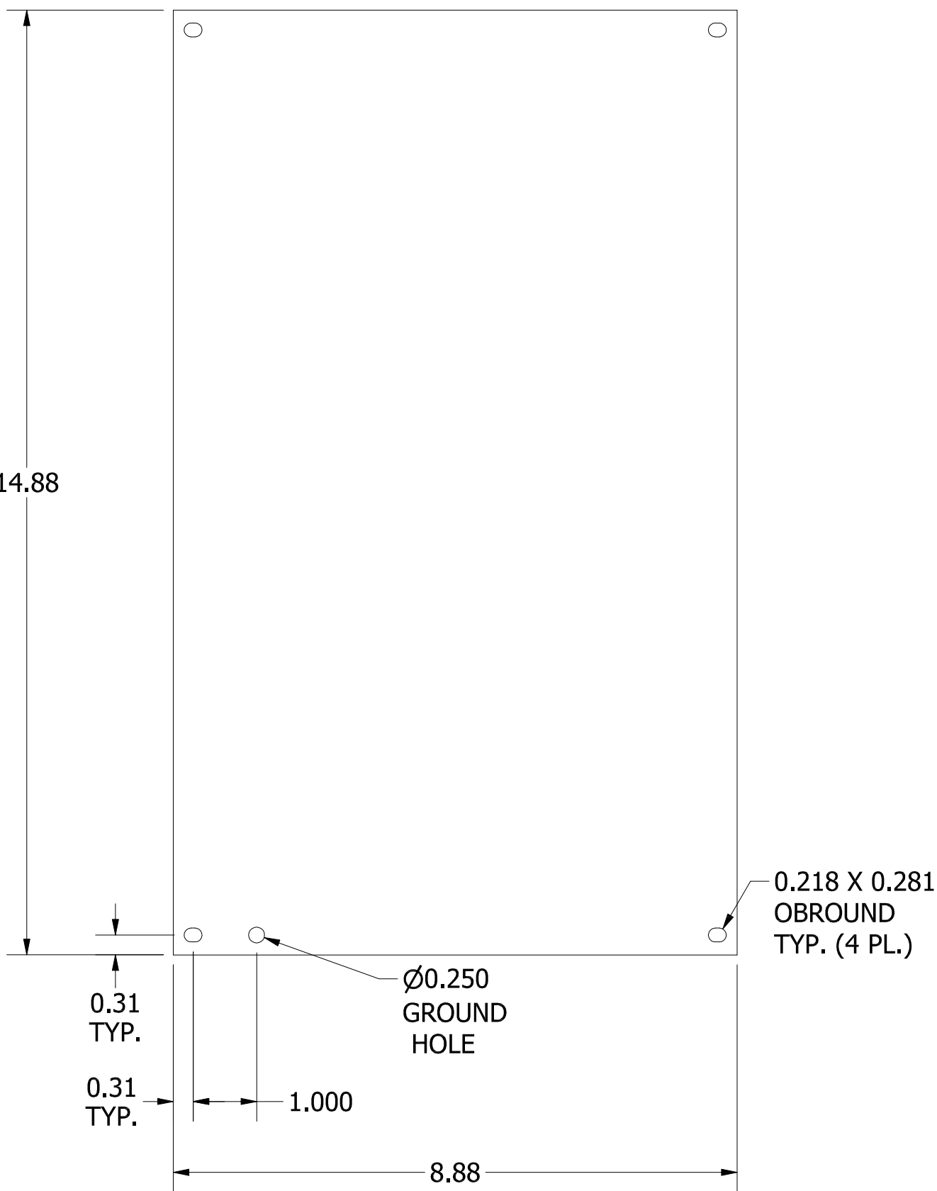
FRONT VIEW
