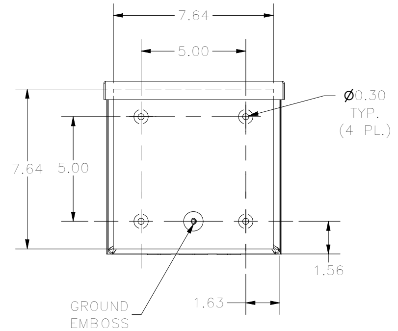
BACK VIEW
