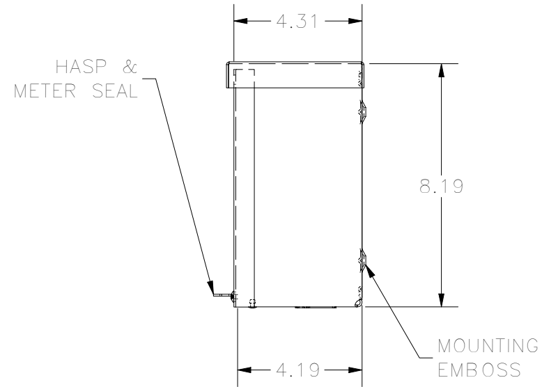
RIGHT VIEW
