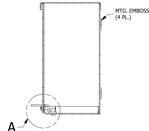
SECTION A-A (INSIDE LEFT OF ENCL.)
