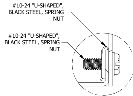
DETAIL A (2 PL.) (LID ATTACHMENT DETAIL)
