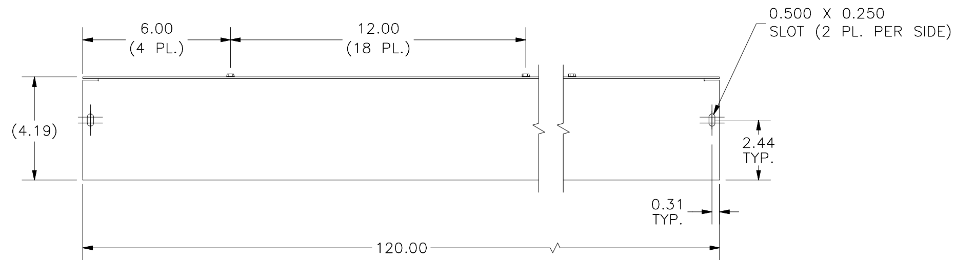
FRONT VIEW
