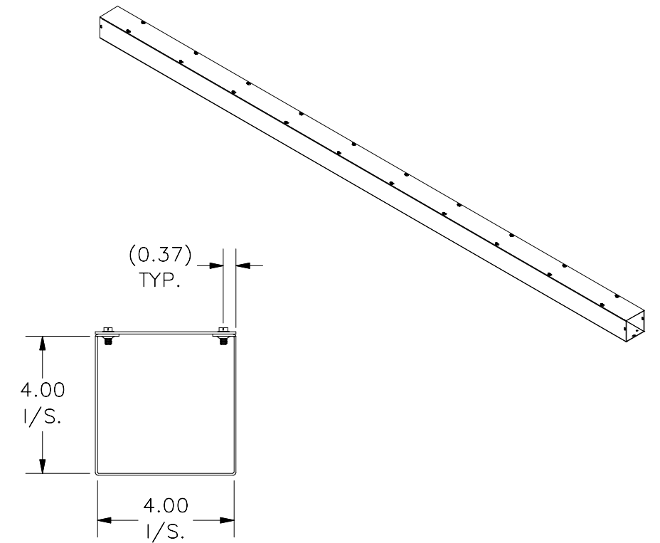
RIGHT VIEW
