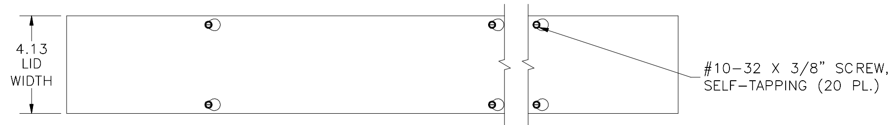
TOP VIEW
