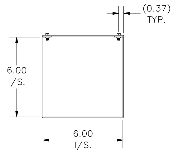
RIGHT VIEW
