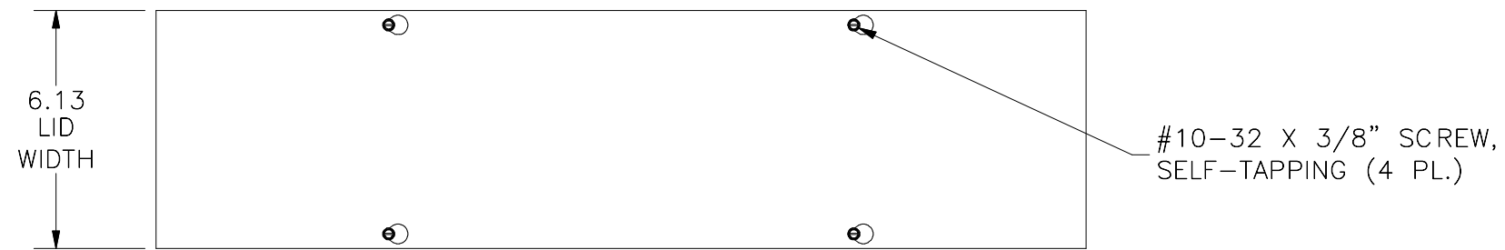
TOP VIEW
