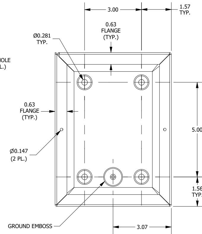
FRONT VIEW LID REMOVED
