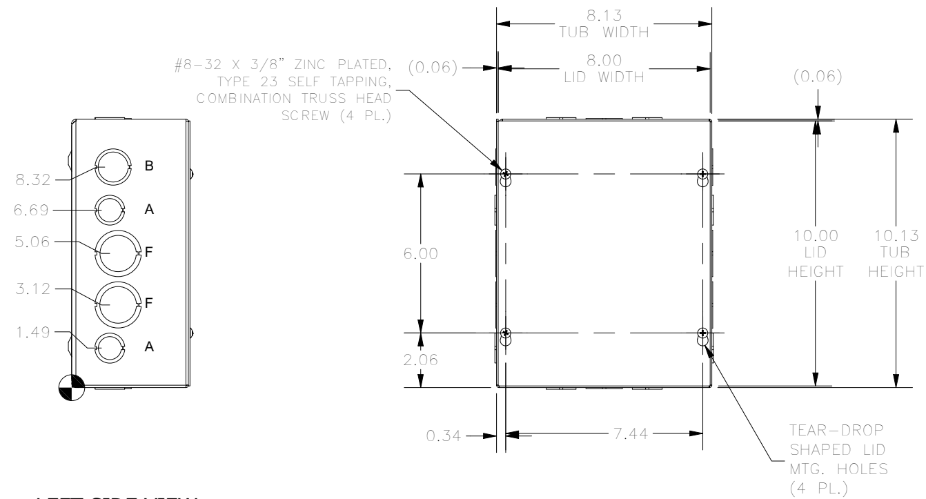
FRONT VIEW
