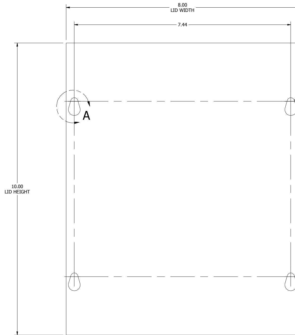
FRONT VIEW
