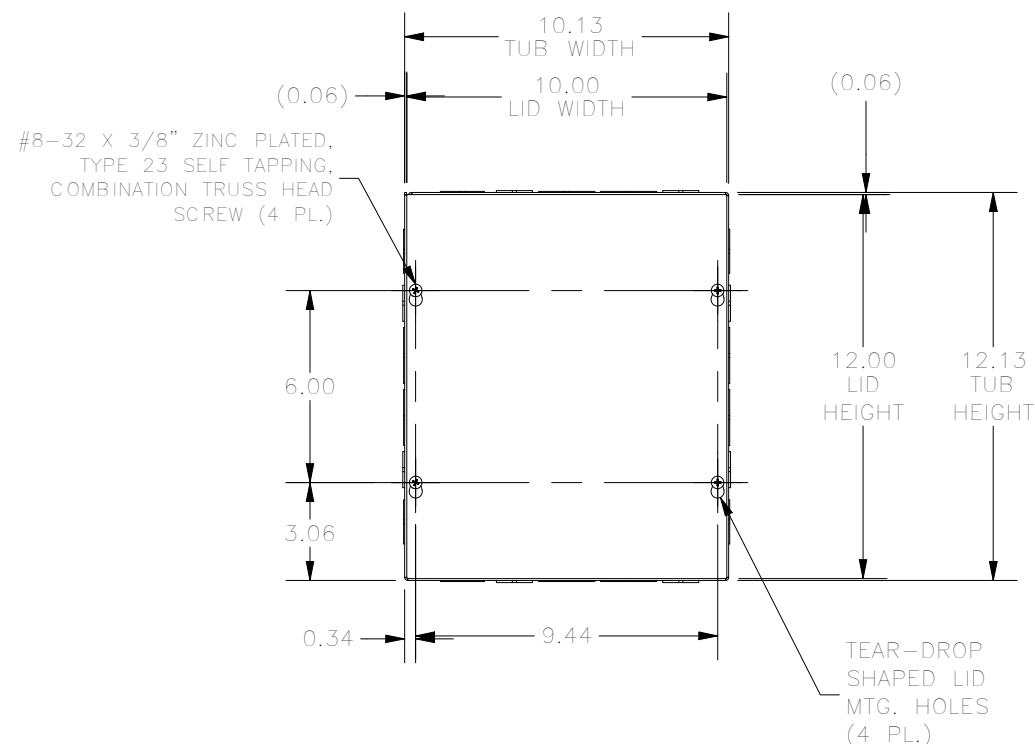
FRONT VIEW
