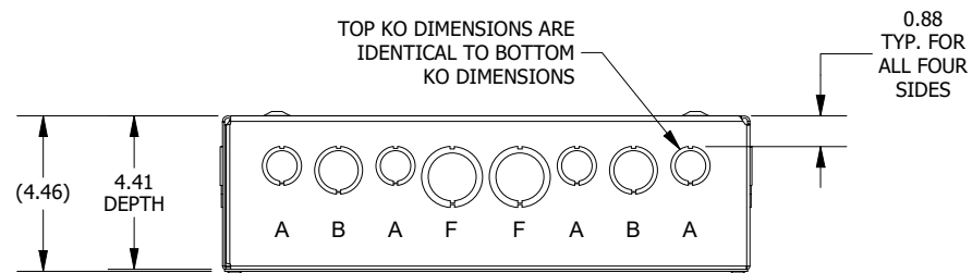
TOP VIEW
