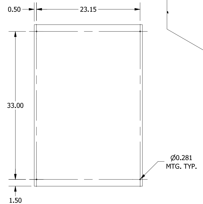
BACK VIEW
