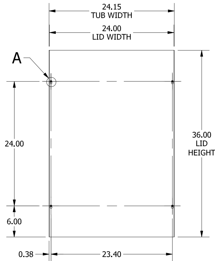
TOP VIEW
