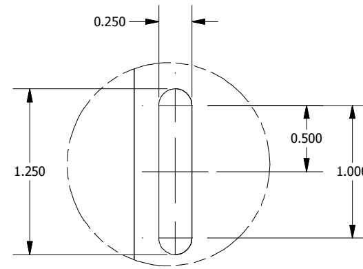
DETAIL A (14 PL.) (SLOT DETAIL)
