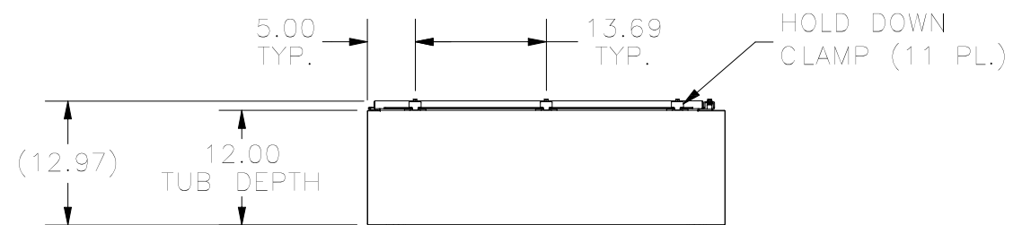
BOTTOM VIEW
