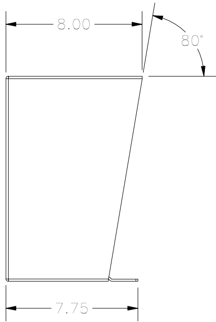
LEFT VIEW
