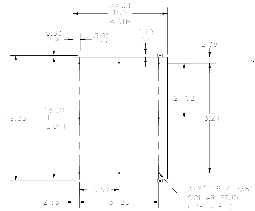
SECTION A-A (INSIDE BACK OF TUB)
