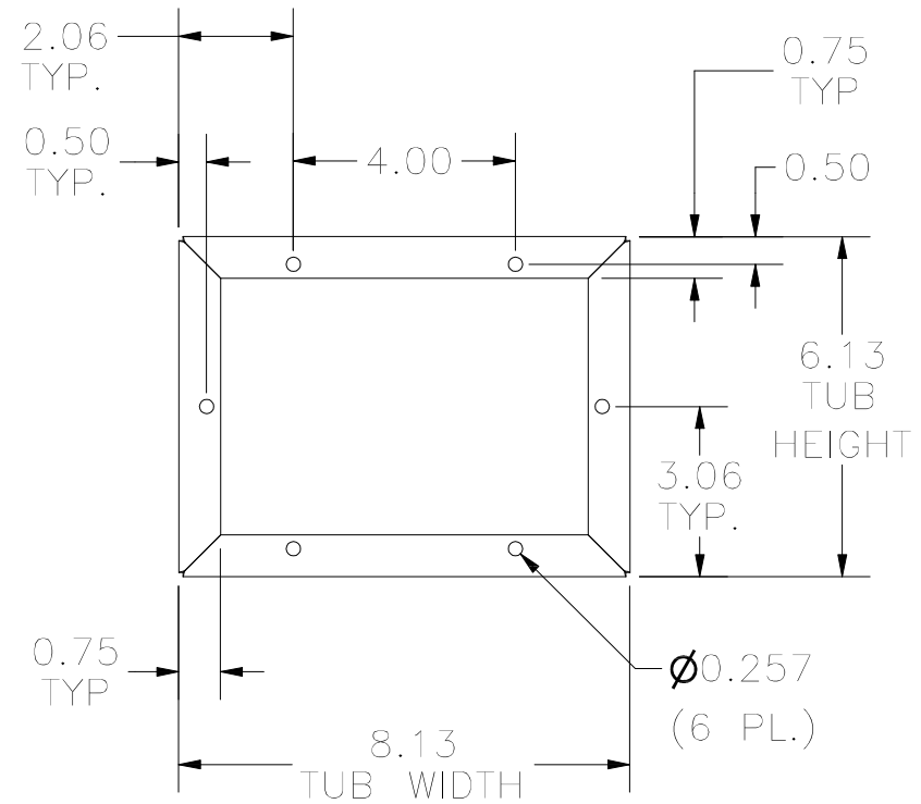
FRONT VIEW OF TUB
