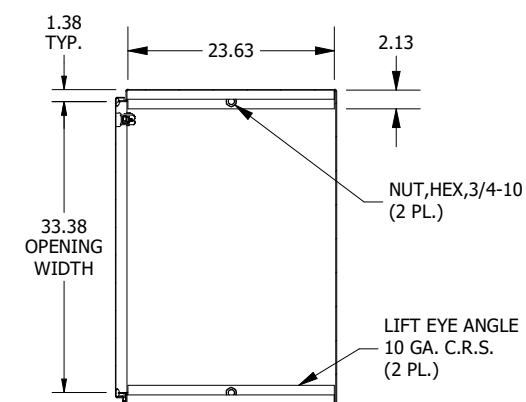
SECTION C-C (INSIDE TOP VIEW OF ENCLOSURE)
