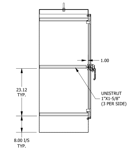
SECTION B-B (INSIDE RIGHT VIEW OF ENCLOSURE)
