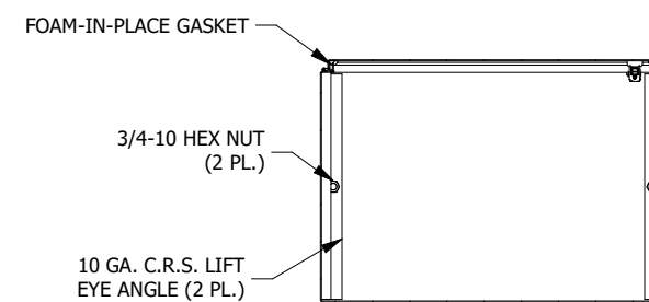
SECTION C-C (INSIDE TOP OF ENCL.)
