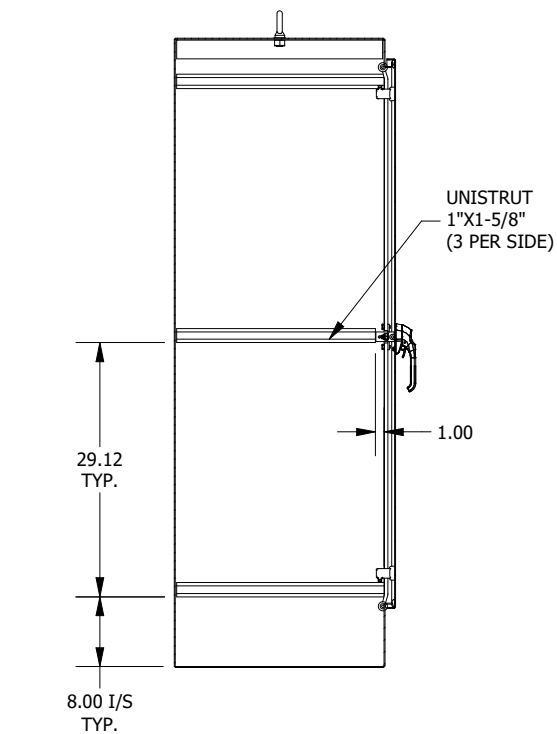
SECTION B-B (INSIDE RIGHT VIEW OF ENCLOSURE)
