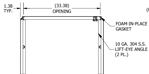
SECTION B-B (INSIDE TOP OF ENCL.)
