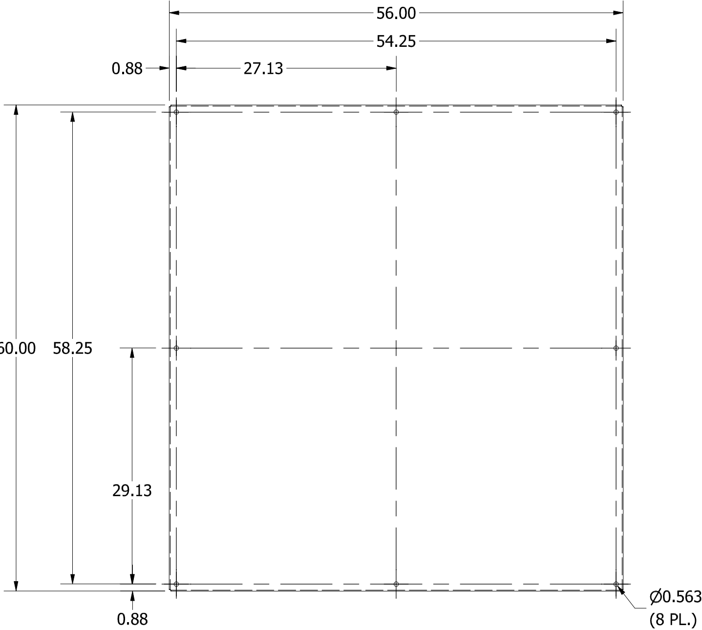
FRONT VIEW
