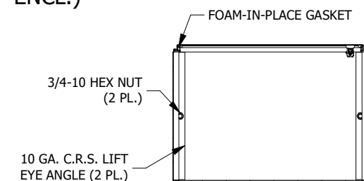
SECTION C-C (INSIDE TOP OF ENCL.)
