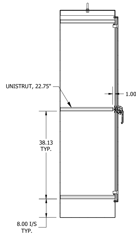
SECTION A-A (INSIDE RIGHT OF ENCL.)
