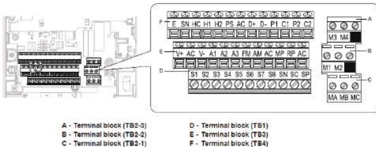
Figure 3 GA800 Control Circuit Terminals
