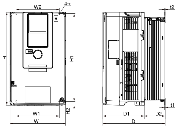
Figure 2: Frames 1 to 3.5
