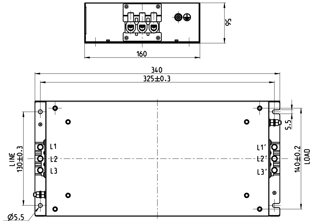
Figure 18: 60 Amp Filter
