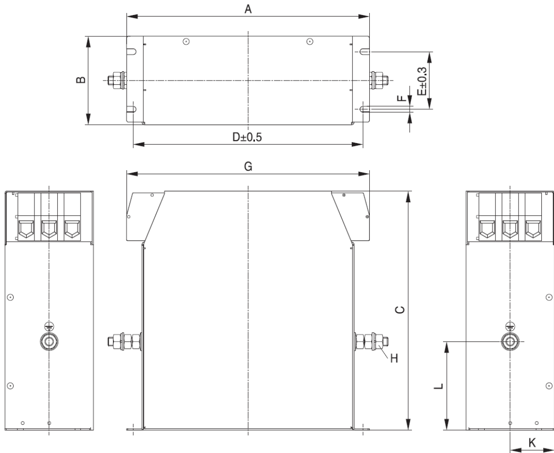
Figure 19: 83 - 180 Amp Filter
