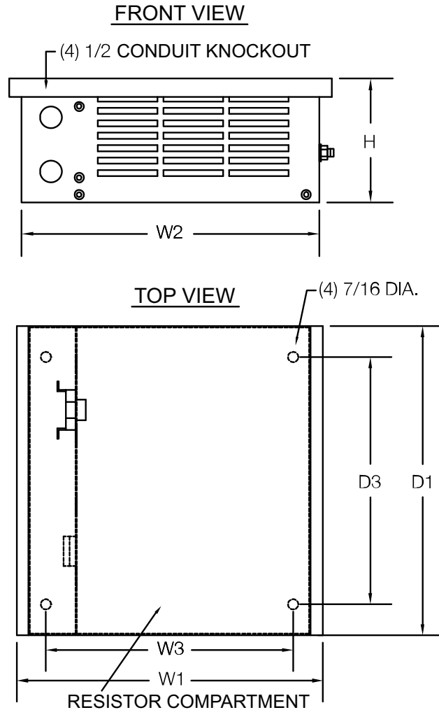
Figure 23: GCE Type Enclosure
